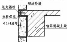
2-2 (梁外保温)
